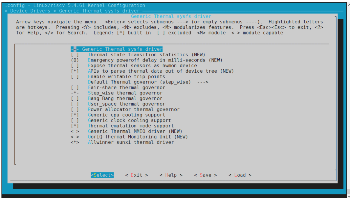
图 3-2: Thermal_menuconfig_T113s3_002
