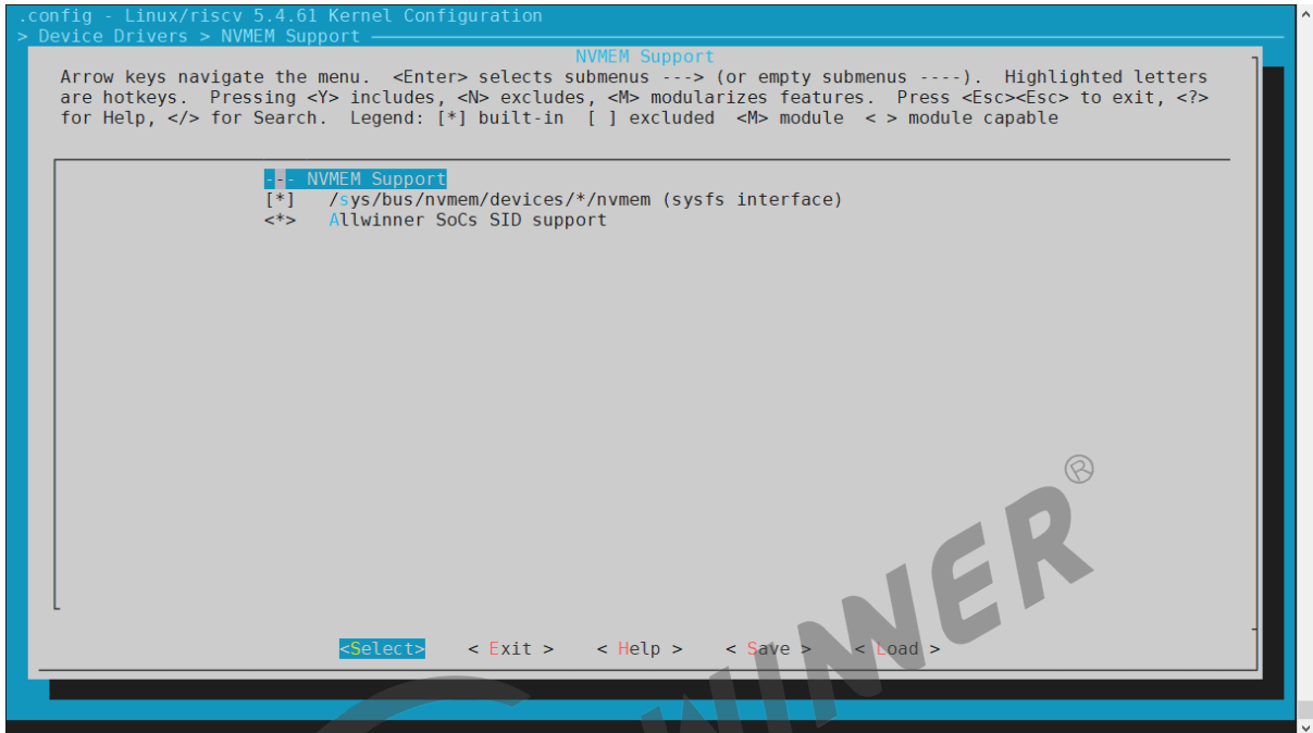
图 3-1: Thermal_menuconfig_T113s3_001
